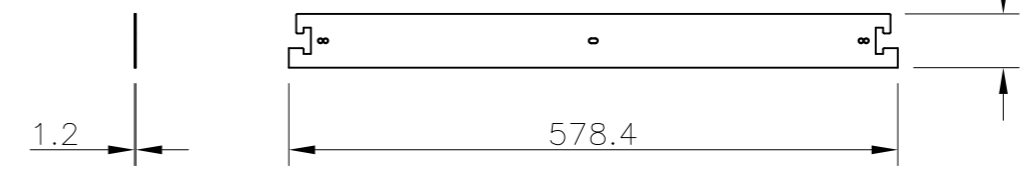
②-2) Multi Brkt Ver < Multi Display > (Brkt-2Ea)
