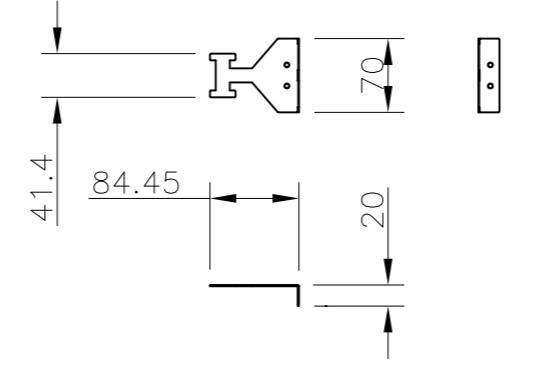
②-3) Multi Brkt Corner & Screw set < Multi Display > (Brkt-2Ea / M4 Screw(L=8- 28Ea))
