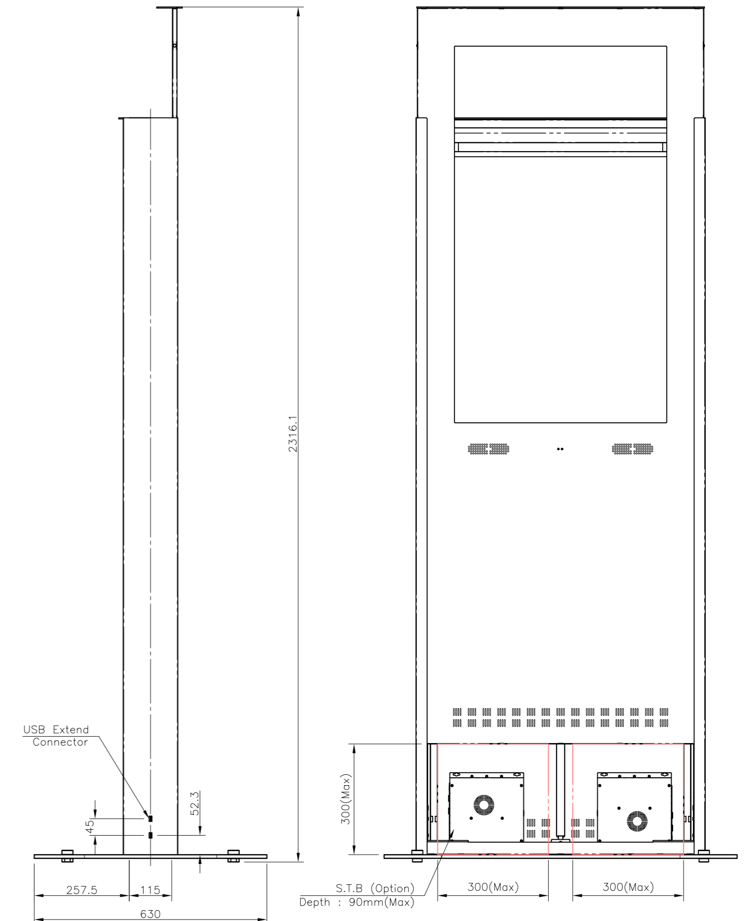
Front-open View
